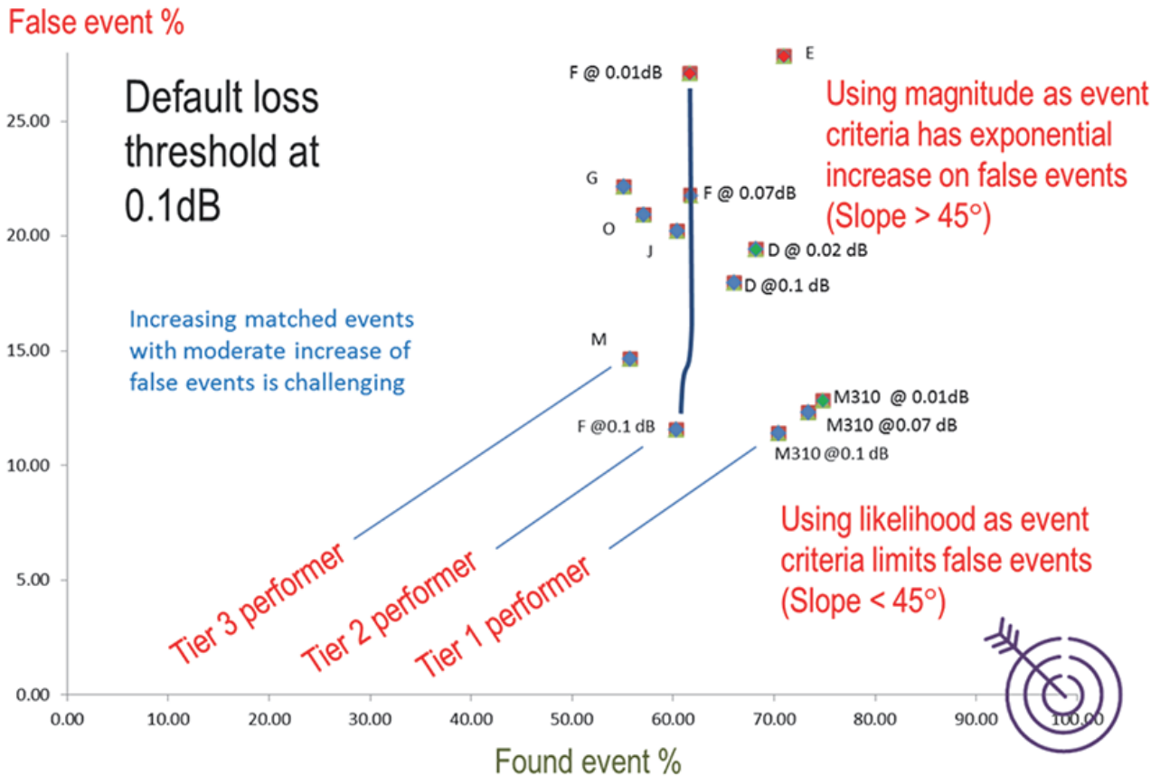
Figure 1 – Event analysis comparison of OTDRs
