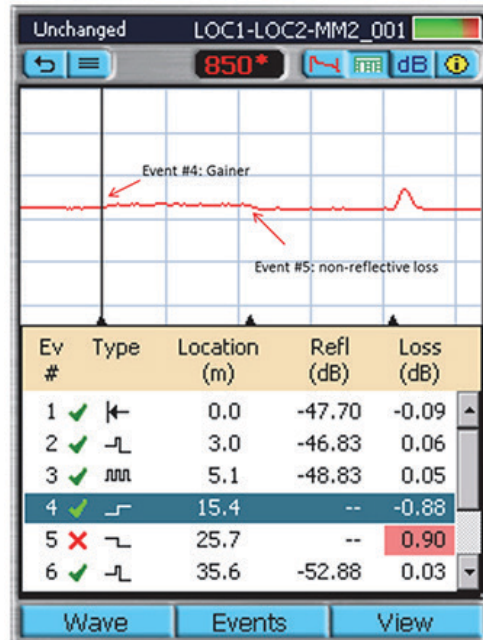
Figure 9 – Zoomed Gainer and non-reflective loss events
