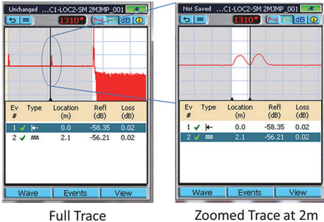
Figure 5 – Closely spaced events; M310 testing a short 2 m jumper cable's performance
