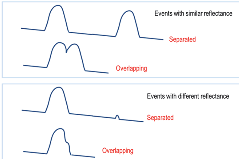
Figure 4 – Closely spaced events
