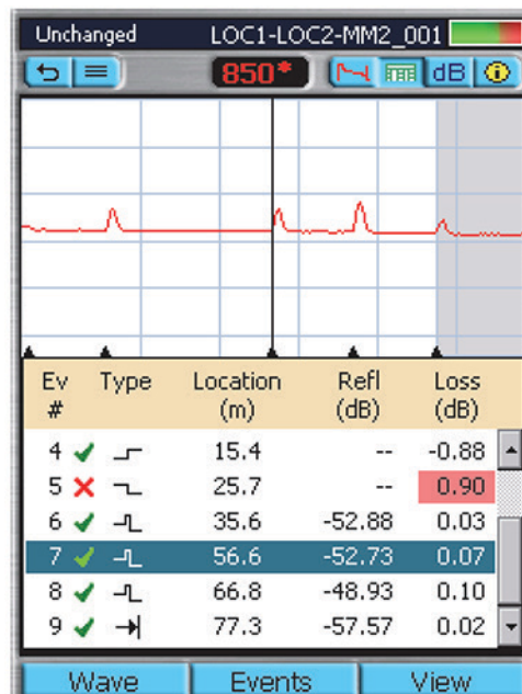
Figure 10 – Data center network zoomed end portion
